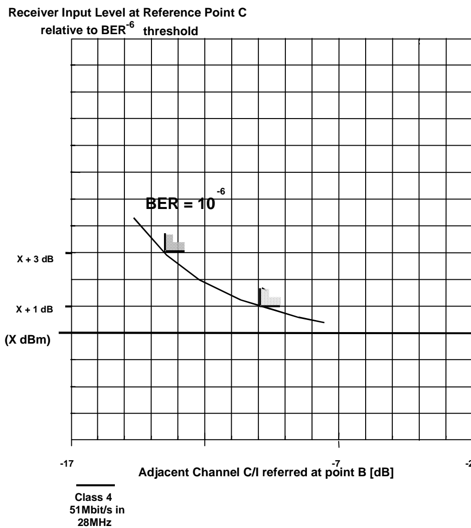
Figure A.5.2b: First adjacent channel interference threshold degradation
