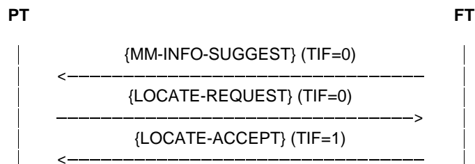
Figure H.3: Location update procedure
