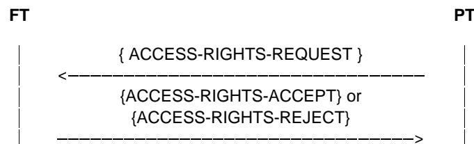
Figure 118: Obtaining of Access Rights
