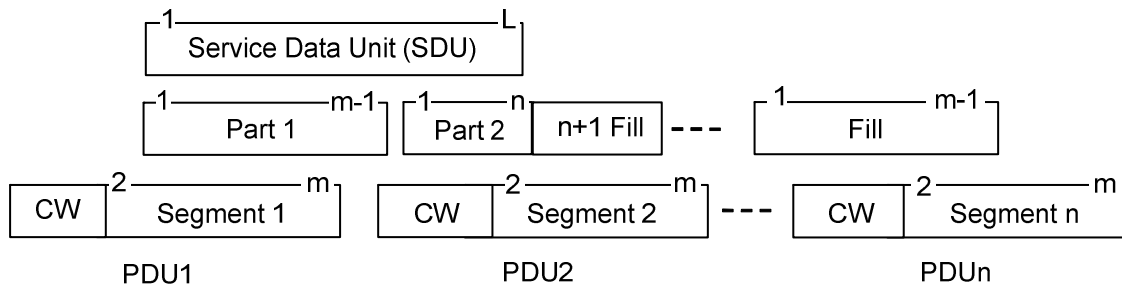
Figure 11.14.2.0.1: LU12 procedures
