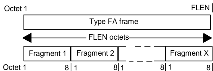
Figure 6.1.4.1.1: C F /CL F logical channel fragmentation
