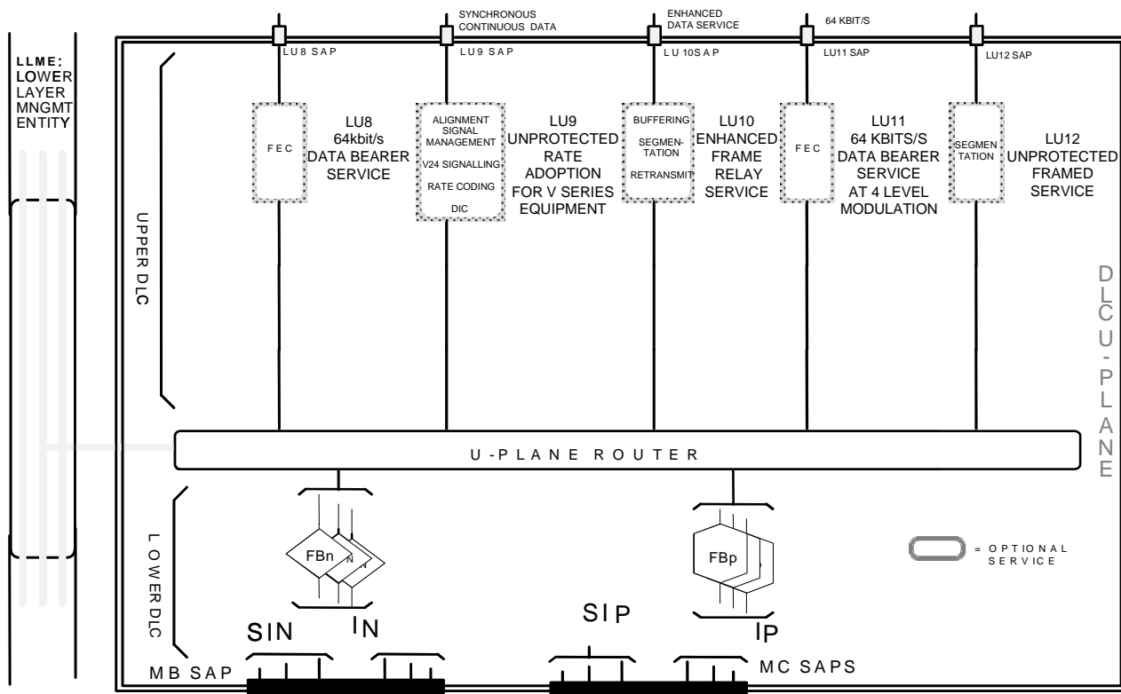
Figure 4.3.1: U-plane model
