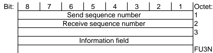
Figure 12.4.1.1: Frame format type FU3a
