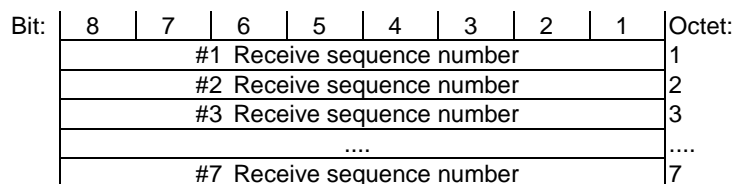
Figure 12.7.1.2: Frame format type FU6b
