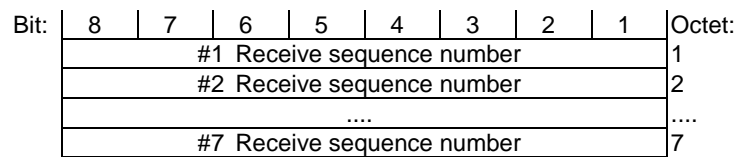
Figure 12.4.1.2: Frame format type FU3b
