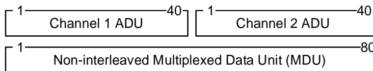
Figure 11.6.3.3.1: Example of non-interleaved packing (MCS Ref: N2/32)
