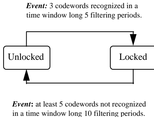
Figure 11.11.2.2.1: Receiver side states
