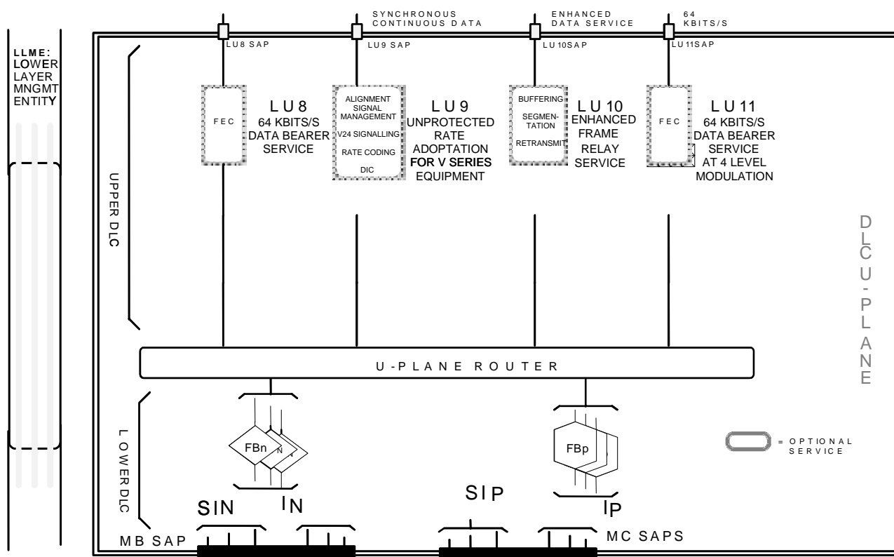
Figure 4.3.1: U-plane model
