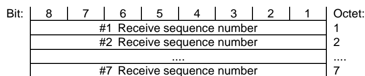
Figure 12.5.1.2: Frame format type FU4b
