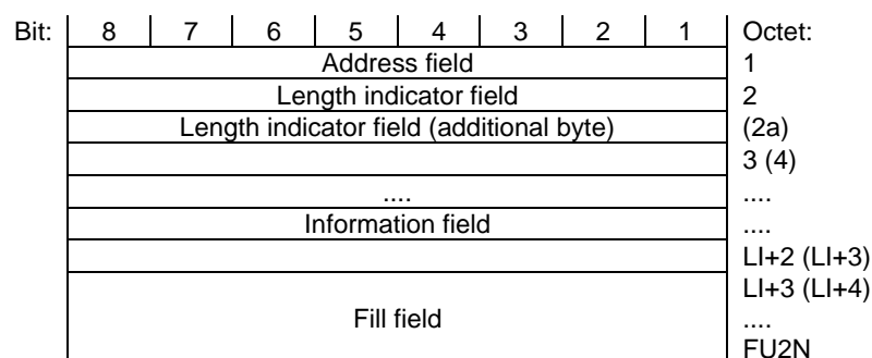
Figure 12.3.1.1: Frame Format Type FU2
