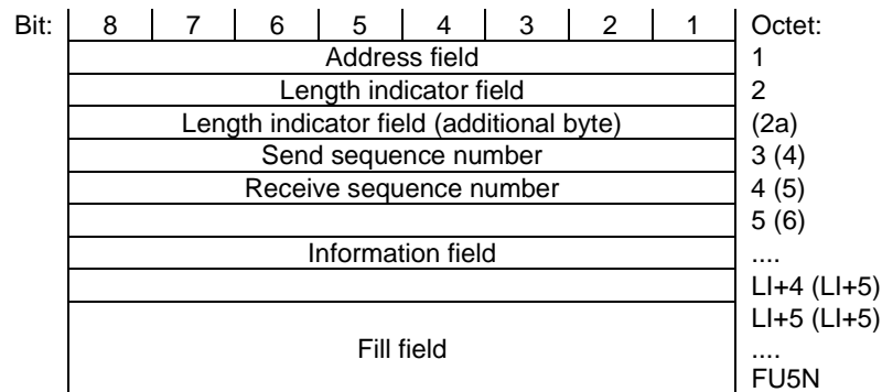
Figure 12.6.1.1: Frame format type FU5a
