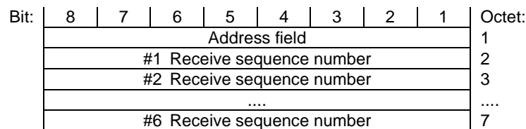
Figure 12.6.1.2: Frame format type FU5b
