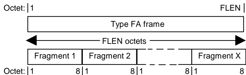
Figure 6.1.4.1.1: C_F/CL_F logical channel fragmentation
