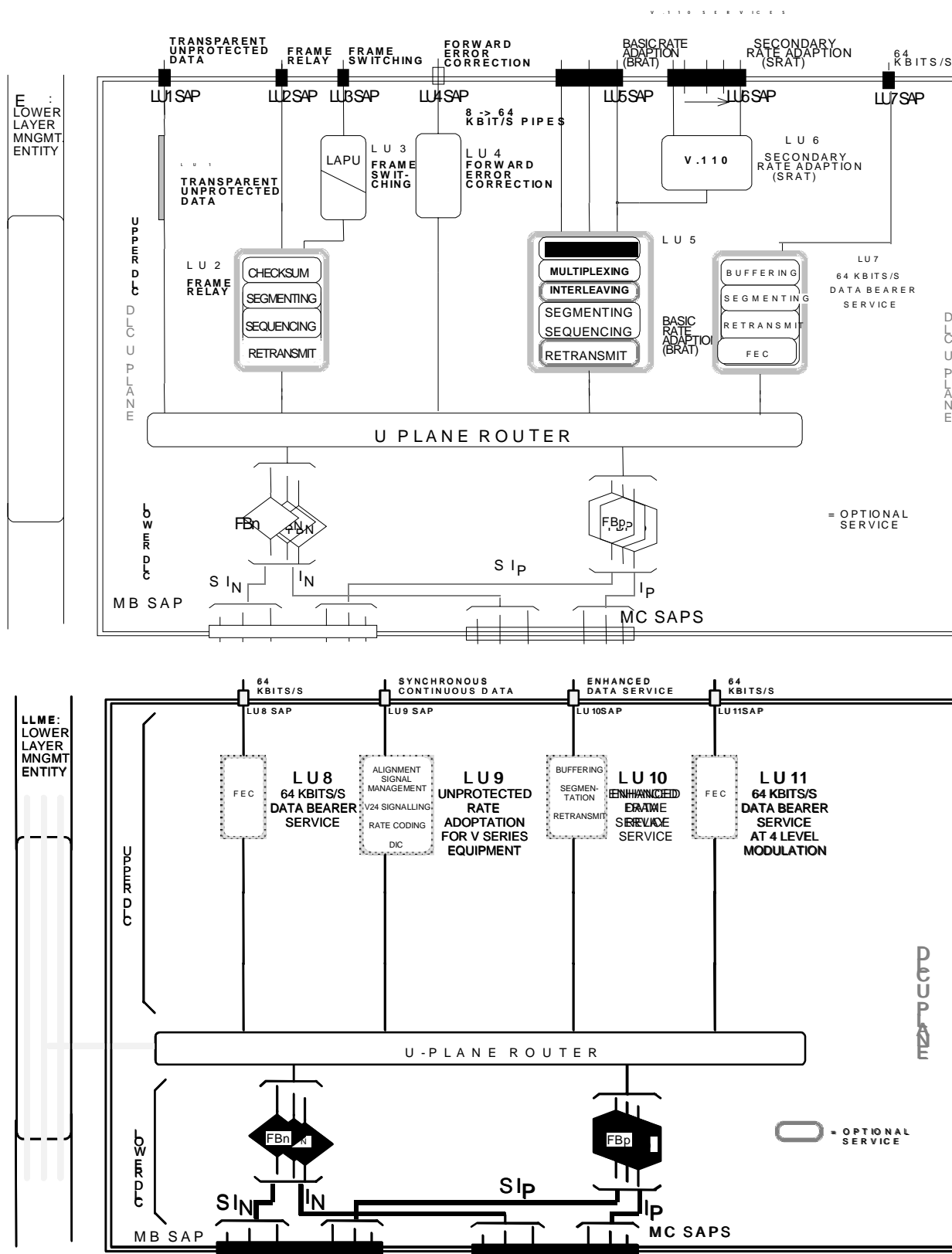
Figure 4.3.1: U-plane model
