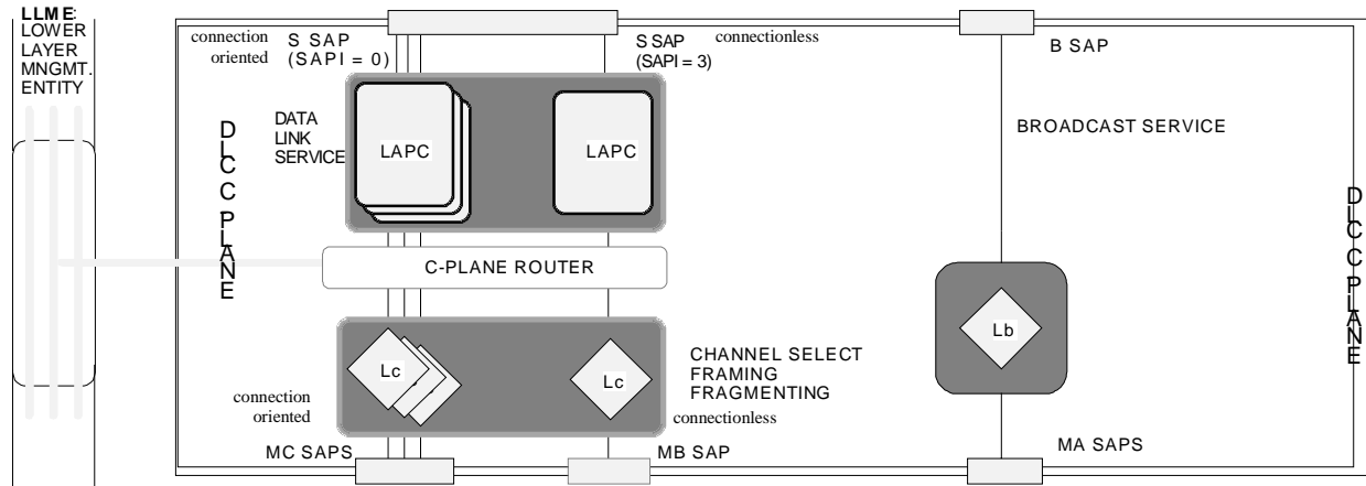
Figure 4.2.1: C-plane model
