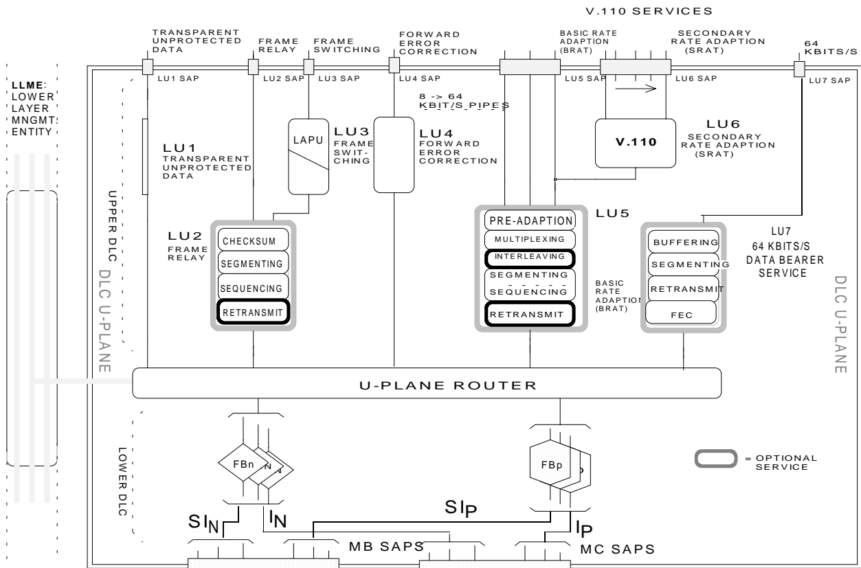
Figure 2: U-plane model
