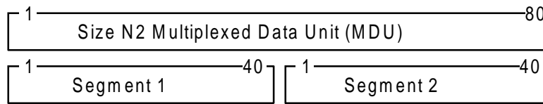
Segmentation of Size N2 MDU
