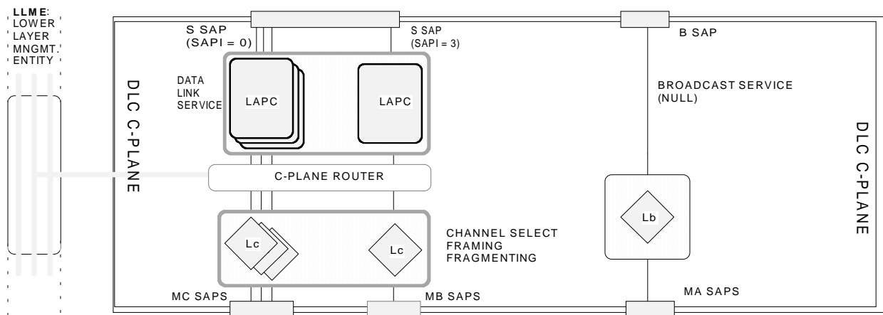
Figure 1: C-plane model
