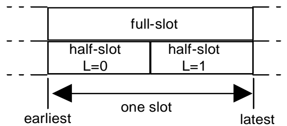
Figure 4.4: Half Slots
