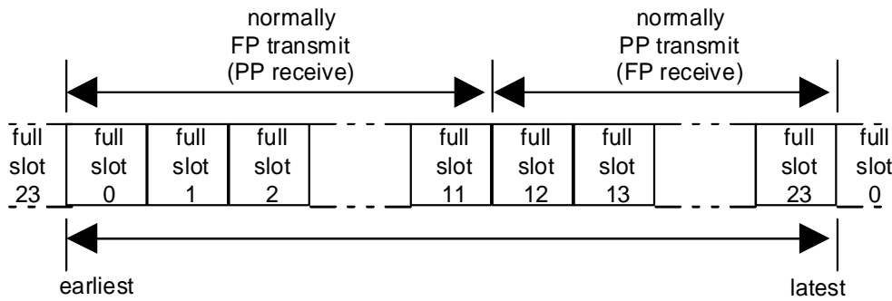
Figure 4.3: Full Slots
