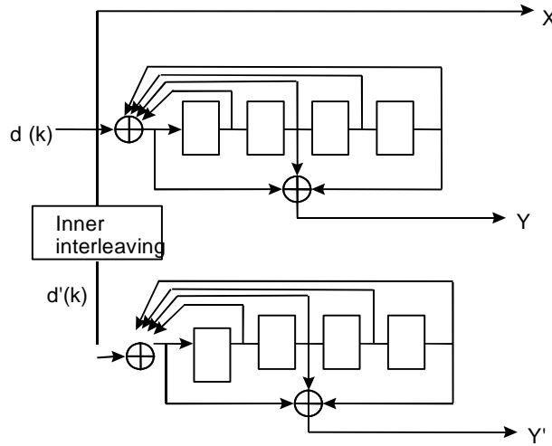
Figure I.4: FOCTC structure
