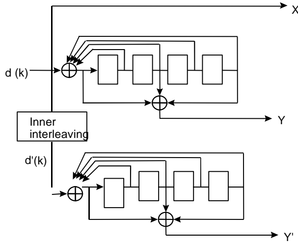
Figure I.4: FOCTC structure
