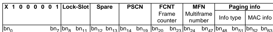
Figure 7.87: "no-emission" mode sync information
