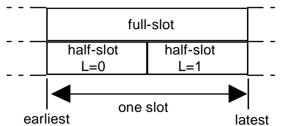
Figure 4.4: Half Slots
