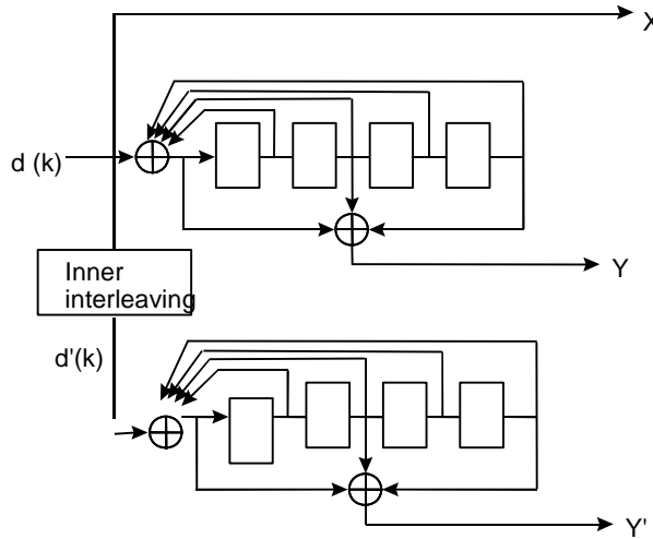
Figure I.4: FOCTC structure
