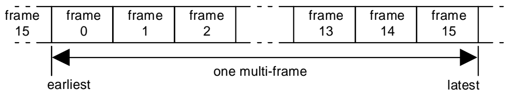
Figure 4.6: Multiframe
