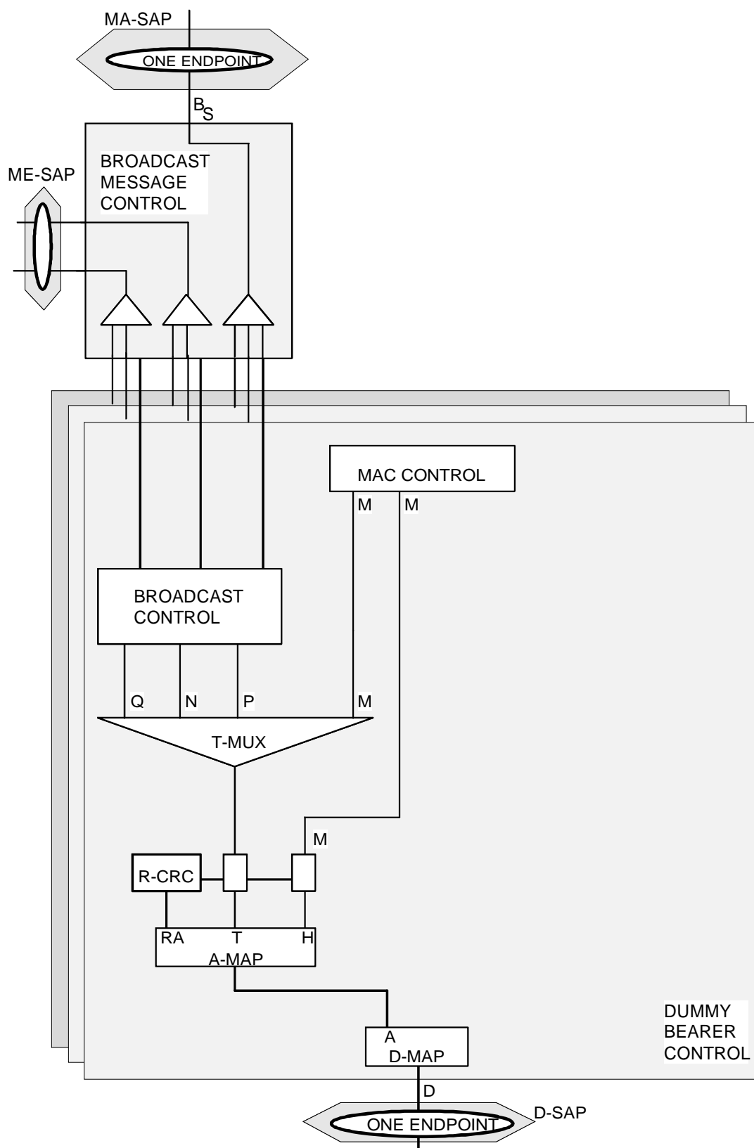
Figure 6.3: DBC multiplexing
