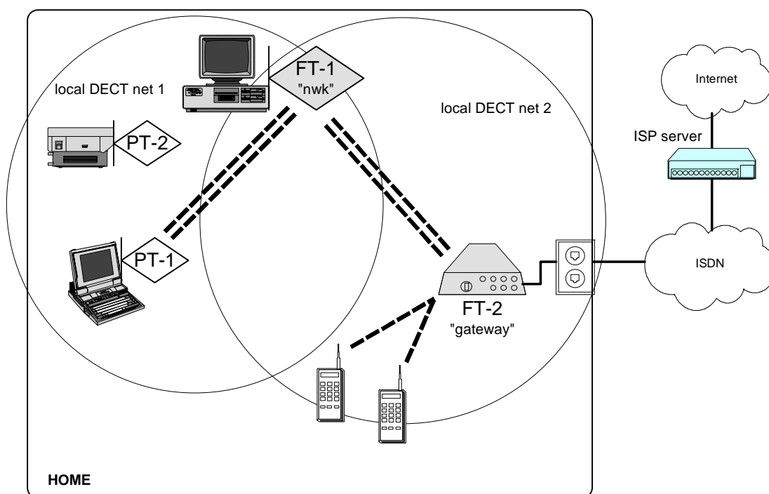
Figure H.1: W-FT2FT communication
