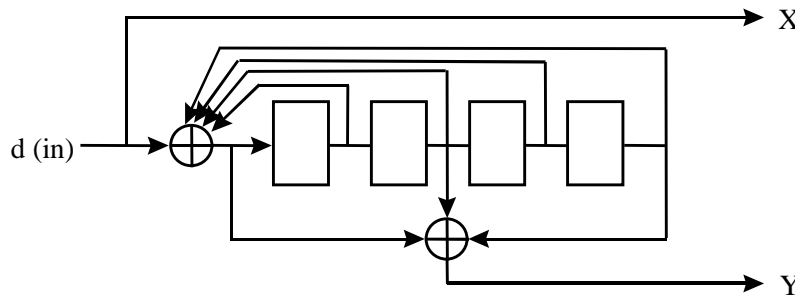
Figure I.3: Recursive Systematic Convolutional (RSC) code
