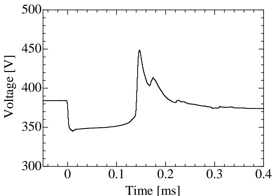
Figure F.3: Example of result of short circuit and voltage transient measurement on simulation circuit described in figure F.2
