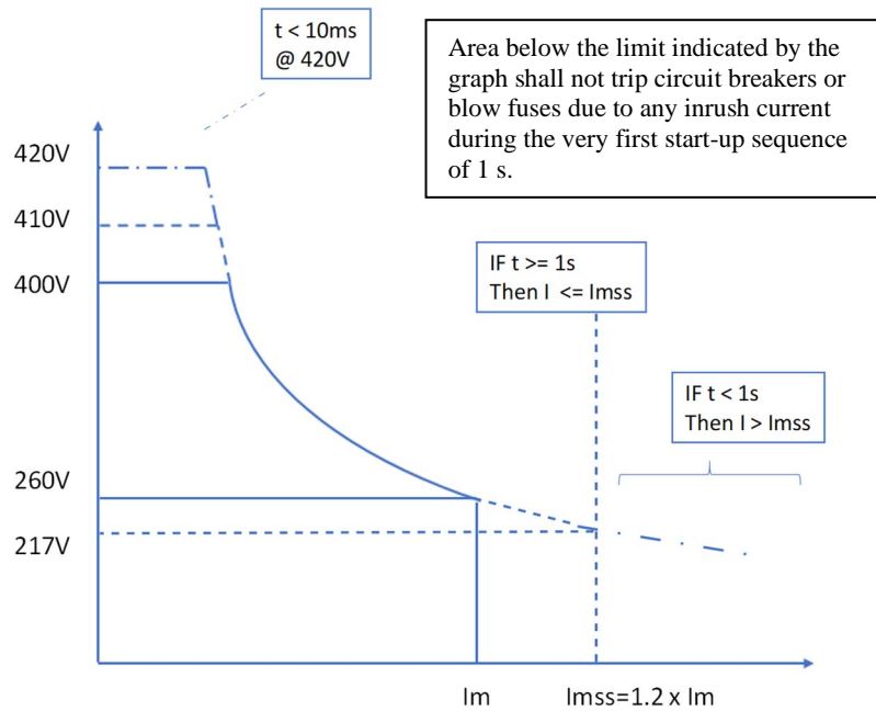
Figure 3: Maximum inrush current characteristics for telecommunications and datacom (ICT equipment > 250 W at U_T )
