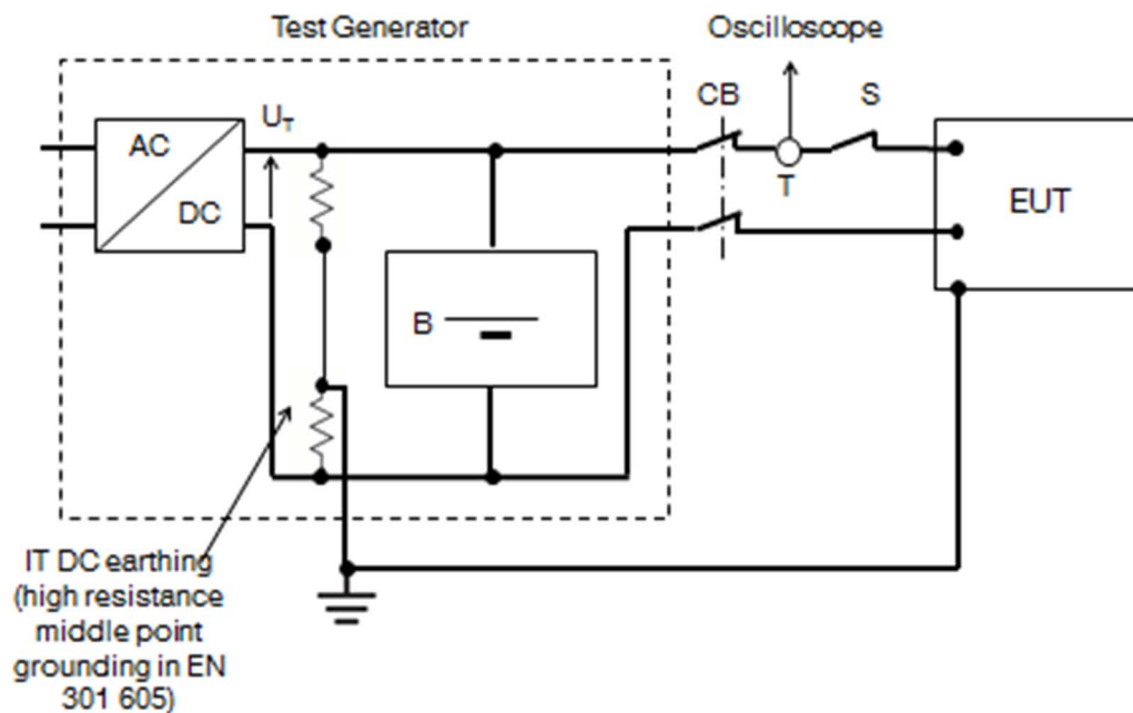
Figure 4: Inrush current test set-up
