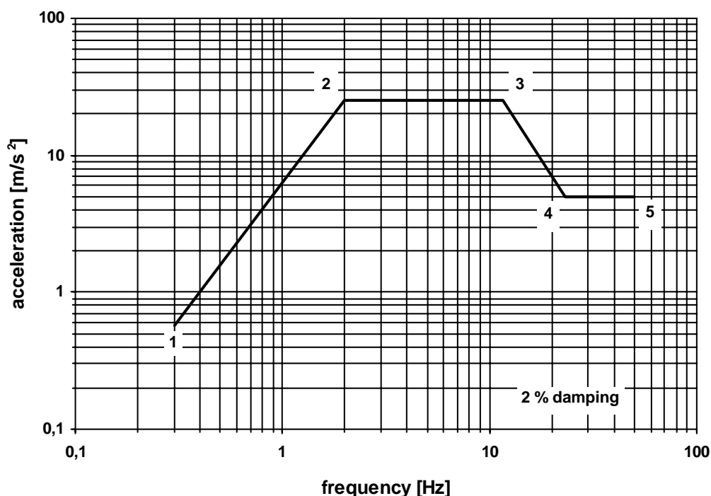
Figure 3: Earthquake Response Spectrum
