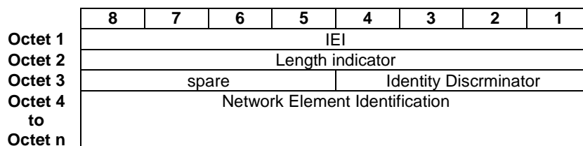
Figure 10.19.1: Network Element Identity IE
