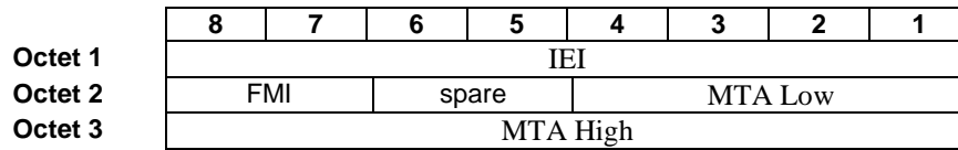
Figure 10.38.1: Multilateration Timing Advance Information
