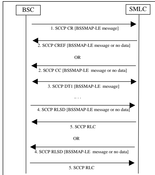
Figure 6.3.3: SCCP Connection Oriented Signaling on Lb Interface for Positioning
