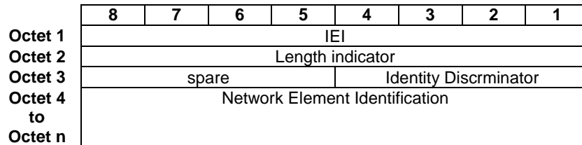
Figure 10.19.1: Network Element Identity IE
