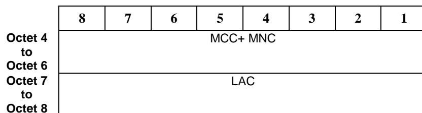
Figure 10.19.4: Coding of Network Element Identification using the MCC + MNC + LAC
