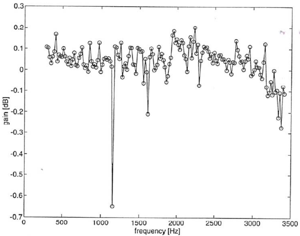
Figure 2: Frequency response in the telephone bandwidth
