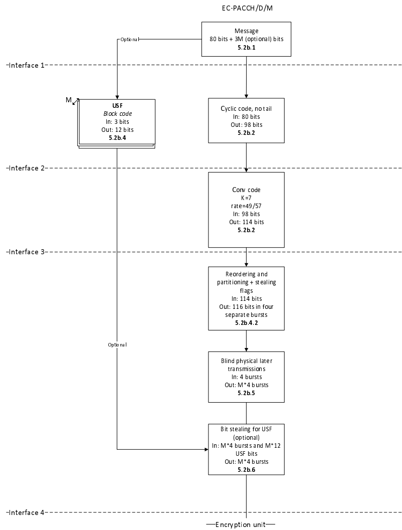
Figure 2ae: Channel Coding and Interleaving Organization for EC-PACCH/D
