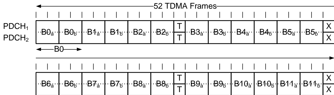
Figure 9: 52- multiframe for PDCHs in BTTI configuration
