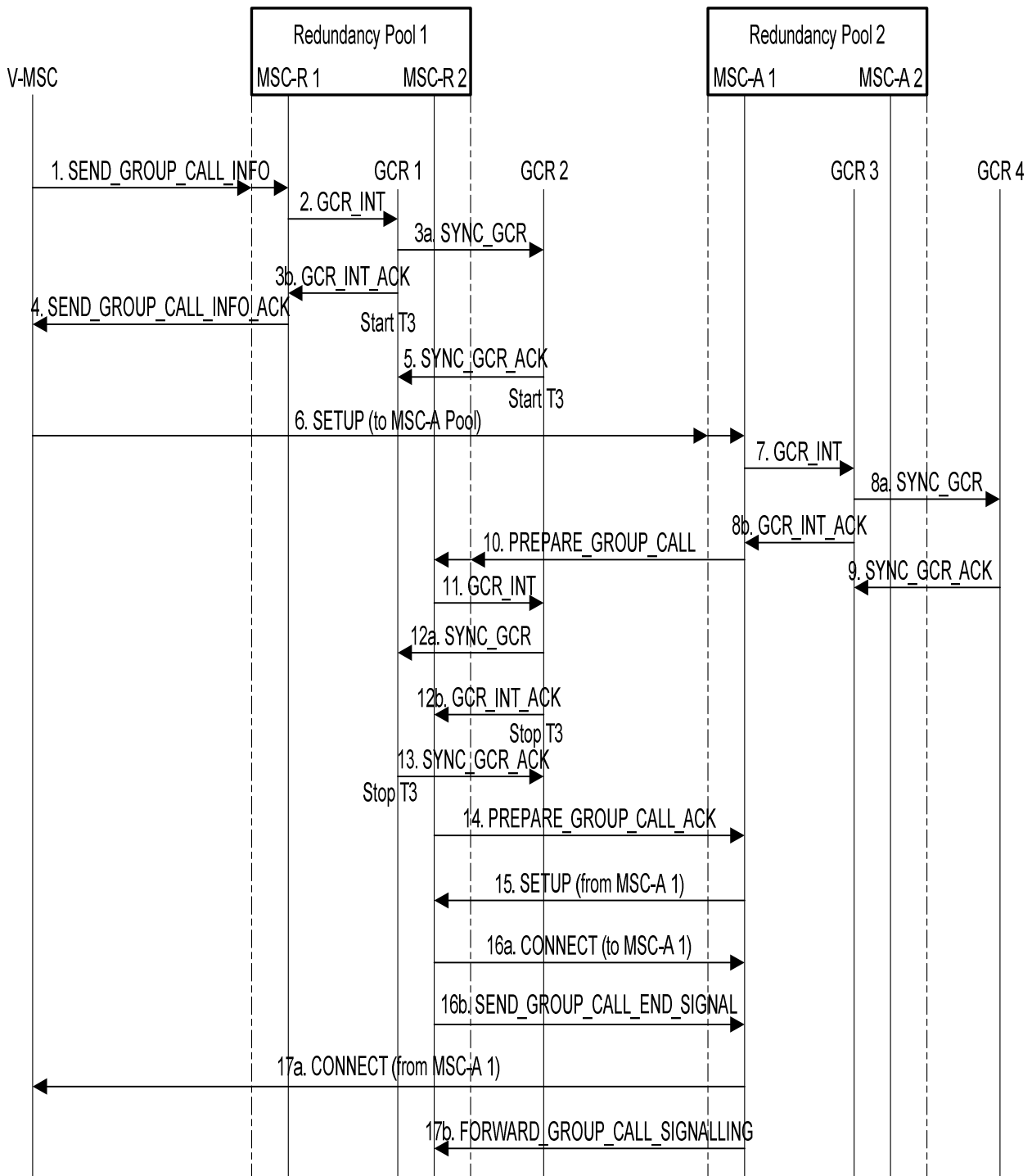
Figure 3c: Signalling information MSC required for establishing voice group calls by a service subscriber in a RANflex configuration with group call redundancy
