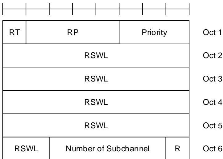
Figure 6.1.3.54-1: Inter-UE Coordination Request MAC CE
