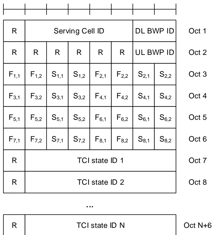
Figure 6.1.3.71-1: Enhanced TCI state activation/deactivation MAC CE for Separate TCI States
