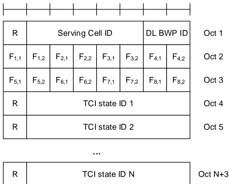
Figure 6.1.3.70-1: Enhanced TCI state activation/deactivation MAC CE for Joint TCI States
