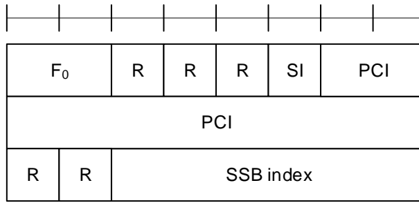
Figure 6.1.3.36-3: Spatial Relation for Resource ID i with SSB
