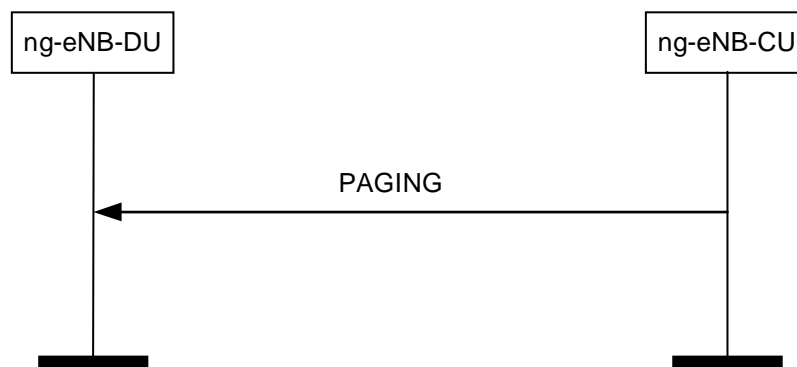
Figure 8.6.1.2-1: Paging procedure. Successful operation.
