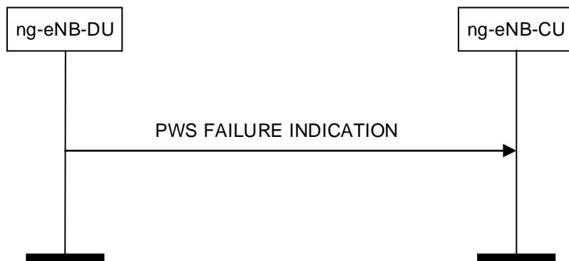
Figure 8.5.4.2-1: PWS failure indication
