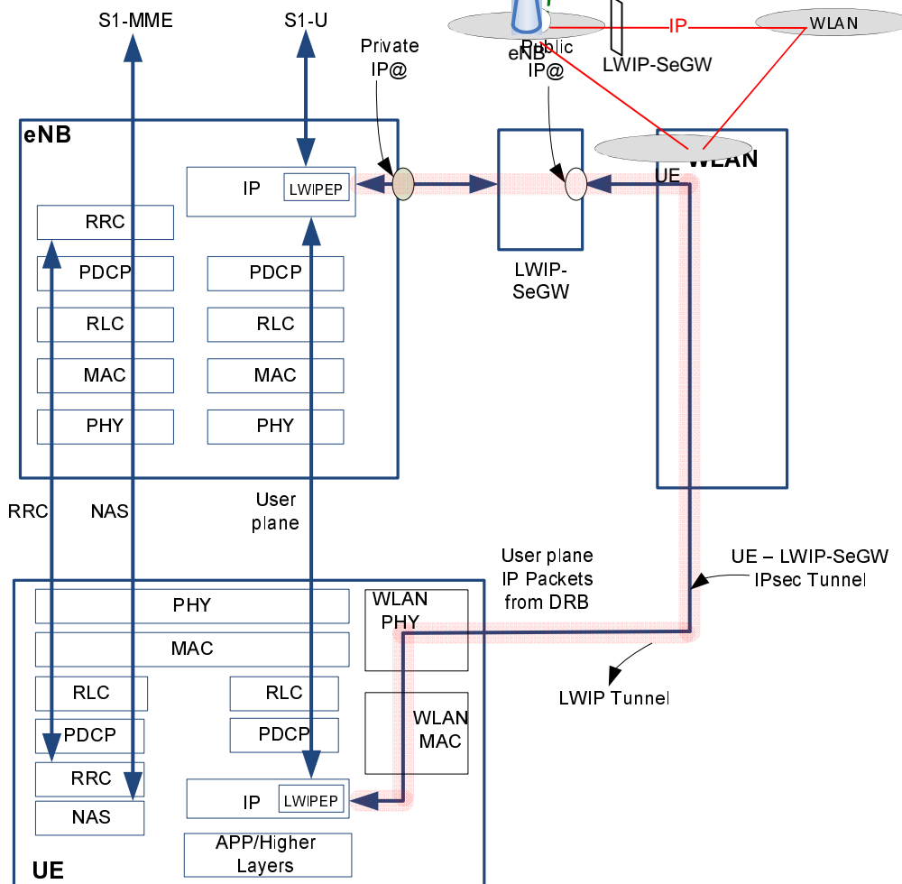
Figure 22A.3-2: LWIP Protocol Architecture
