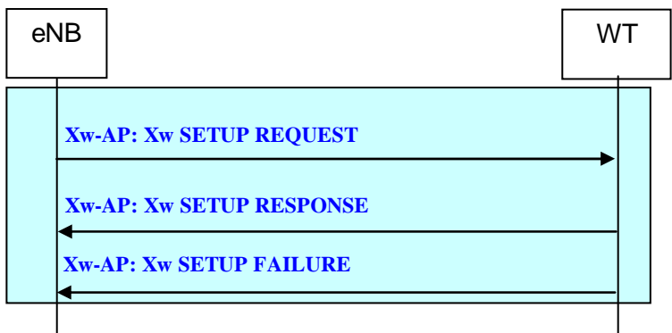
Figure 22B.2.2.9-1: Xw Setup procedure
