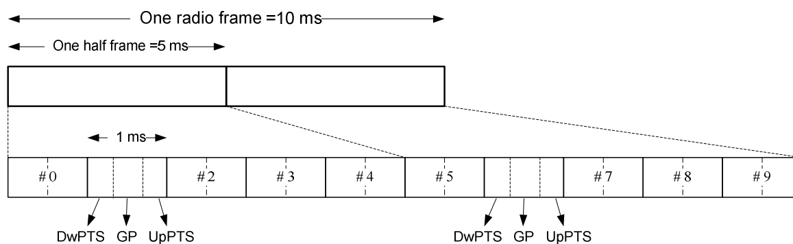
Figure 5.1-2: Frame structure type 2 (for 5ms switch-point periodicity)
