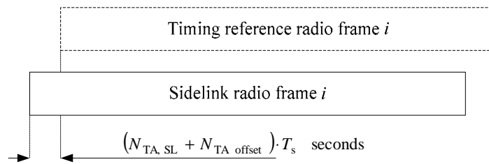
Figure 9.9-1: Sidelink timing relation.
