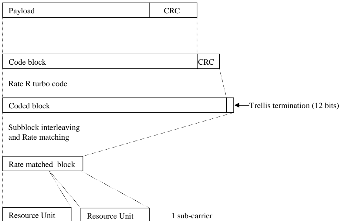
Figure A0-2. Schematic overview of the encoding process for NB-LoT
