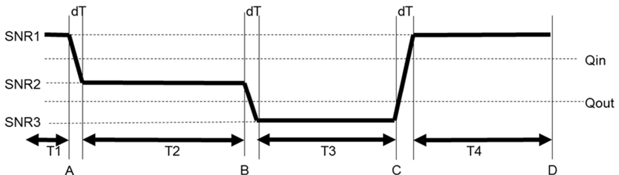
Figure A.7.3.95.1-1: SNR variation for out-of-sync testing
