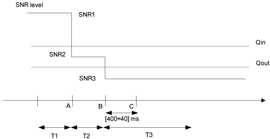
Figure A.7.3.98.1-1: SNR variation for out-of-sync testing
