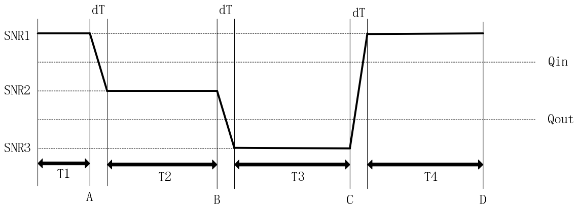
Figure A.7.3.89.1-1: SNR variation for TDD Radio Link Monitoring Test for Out-of-sync in DRX for UE category NB1 In-band mode in enhanced coverage
