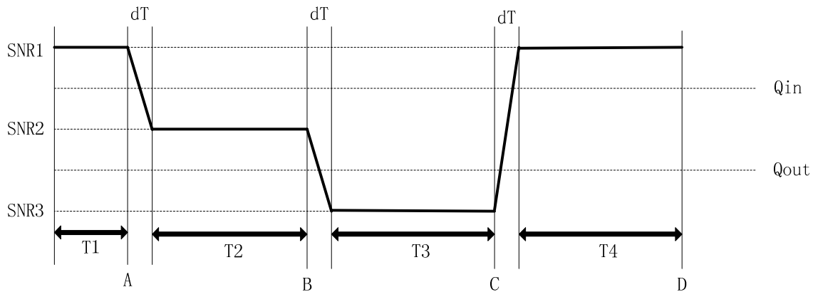
Figure A.7.3.60.1-1: SNR variation for out-of-sync testing in DRX for NB-IoT HD-FDD out-of-sync testing for UE category NB1 configured under normal coverage
