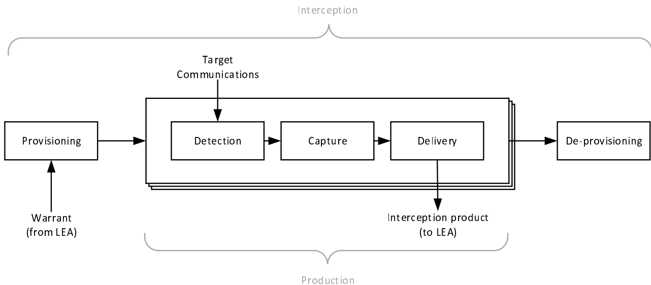
Figure 5.1: Generic Lawful Interception lifecycle
