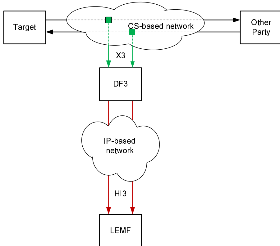
Figure 5.5: IP based handover interface for the CC of a CS intercepts
