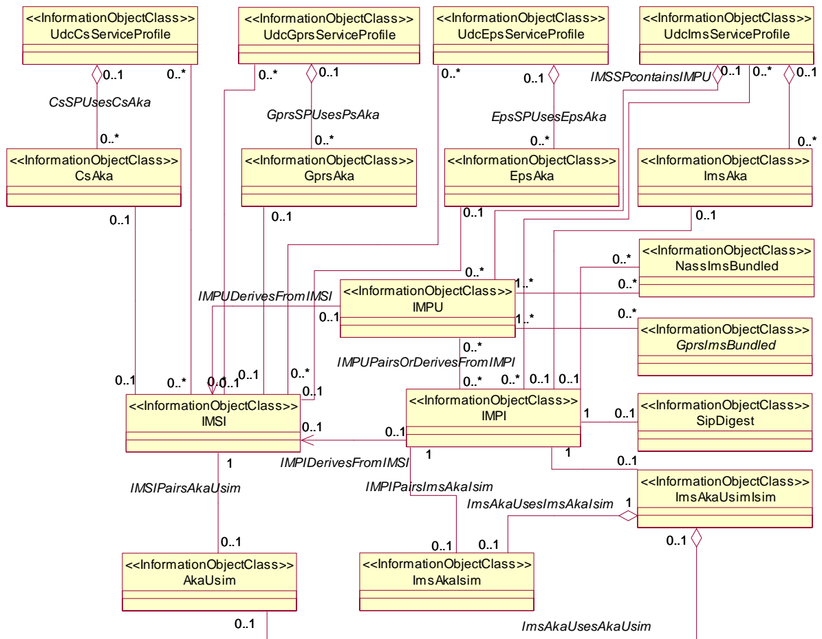
Figure 6.5.2-1: Authentication methods
