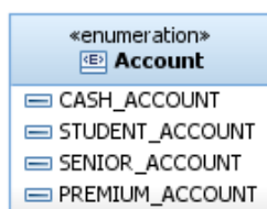
Figure 5.3.5.2-1: <<enumeration>> notation
