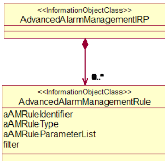
Figure 5.2.1-1: Class Diagram
