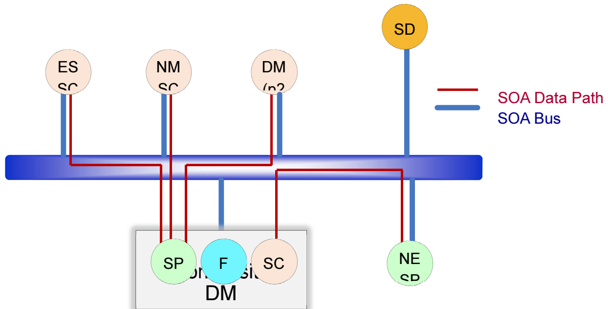
Figure 5: SOA-based representation of the 3GPP Management Reference Model
