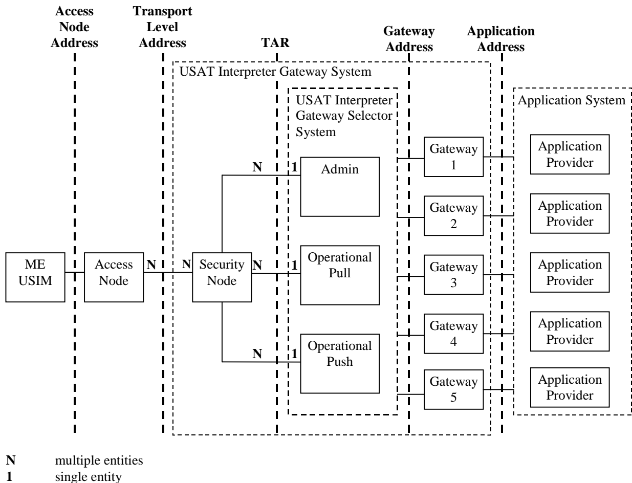
Figure 2: System Architecture
