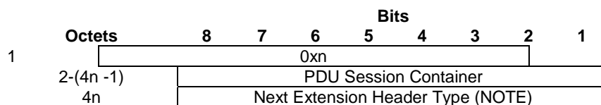
Figure 5.2.2.7-1: PDU Session Container Extension Header
