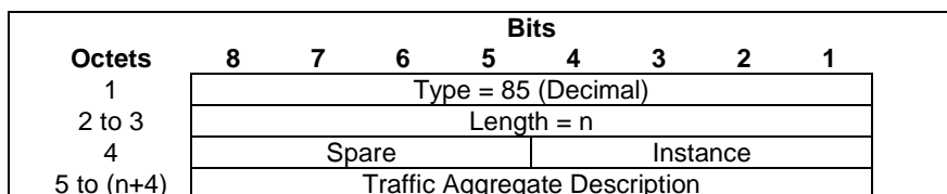
Figure 8.20-1 Traffic Aggregate Description
