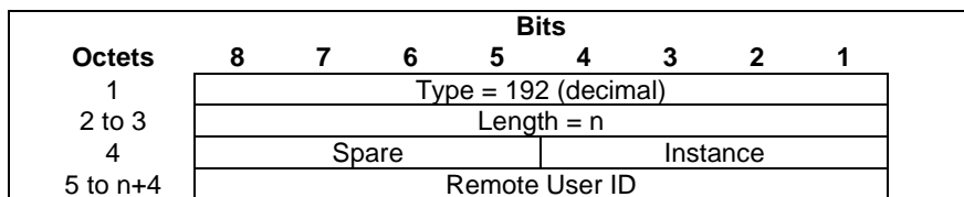
Figure 8.123-1: Remote User ID
