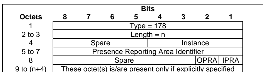
Figure 8.109-1: Presence Reporting Area Information
