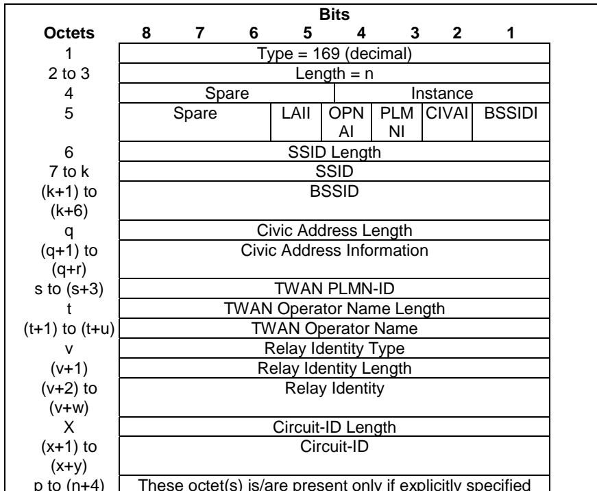
Figure 8.100-1: TWAN Identifier
