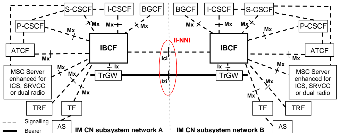
Figure 5.1.1: Inter-IMS Network to Network Interface between two IM CN subsystem networks
