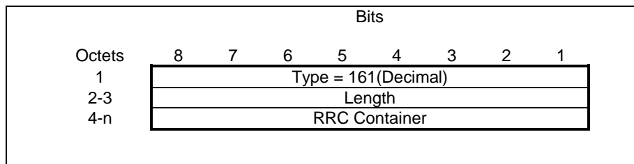
Figure 61a: Source RNC PDCP context info
