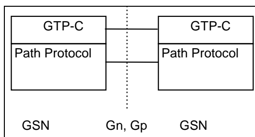
Figure 62: Signalling Plane - Protocol Stack
