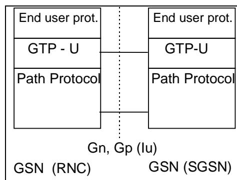
Figure 65: GTP-U - Protocol Stack (GTP-U over the lu in brackets)
