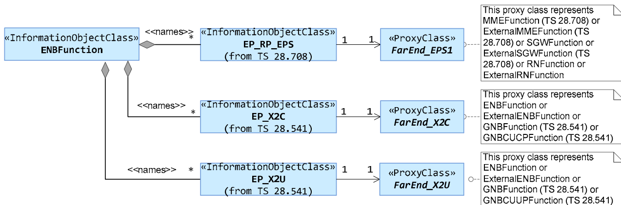
Figure 4.2.1-3: Transport view of E-UTRAN NRM
