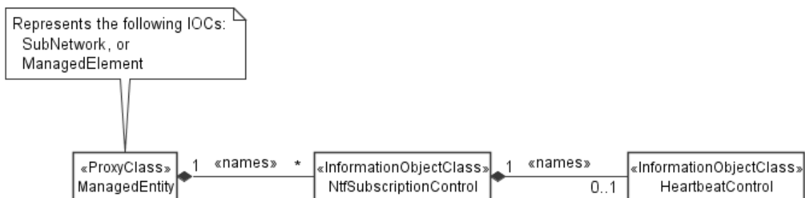
4.2.1-5: Notification subscription and heartbeat notification control NRM fragment
