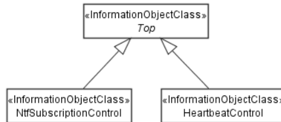
Figure 4.2.2-4: Notification subscription and heartbeat notification control NRM fragment
