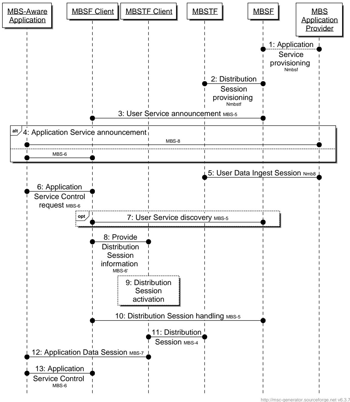
Figure 5.2-1: MBS User Service high-level baseline procedures
