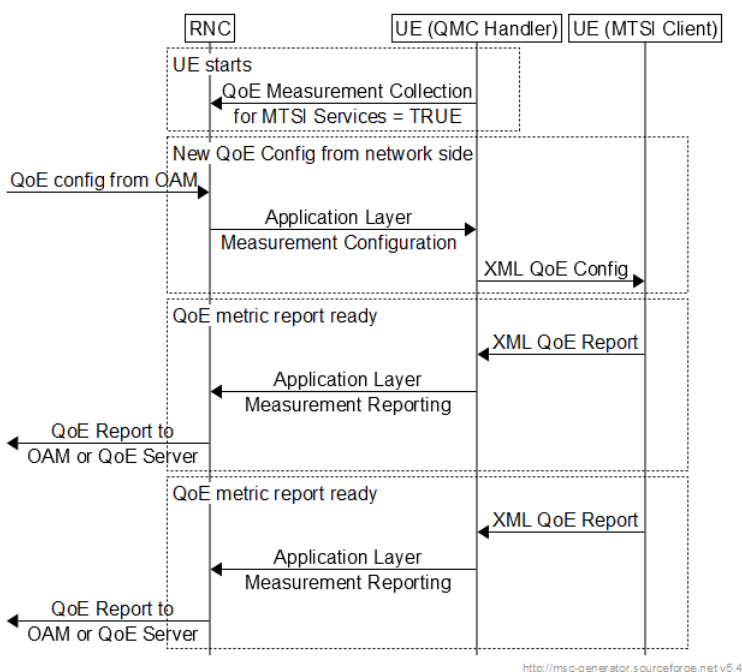
Figure 16.5.1-1: Example signalling diagram for UMTS
