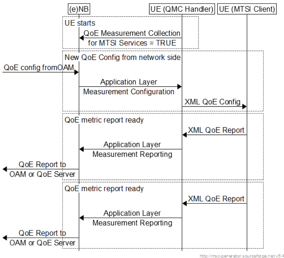
Figure L-1: example signalling diagram
