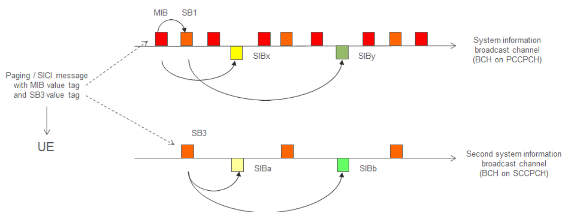
Figure 9.1-2: System information acquisition on system information broadcast channel and second system information broadcast channel.
