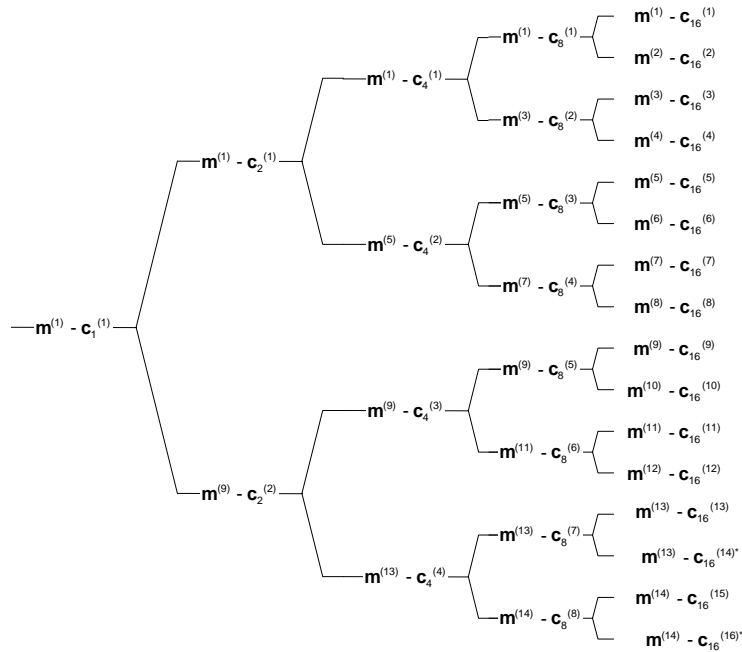
Figure AA.2.2: Association of Midambles to Spreading Codes for K=14
