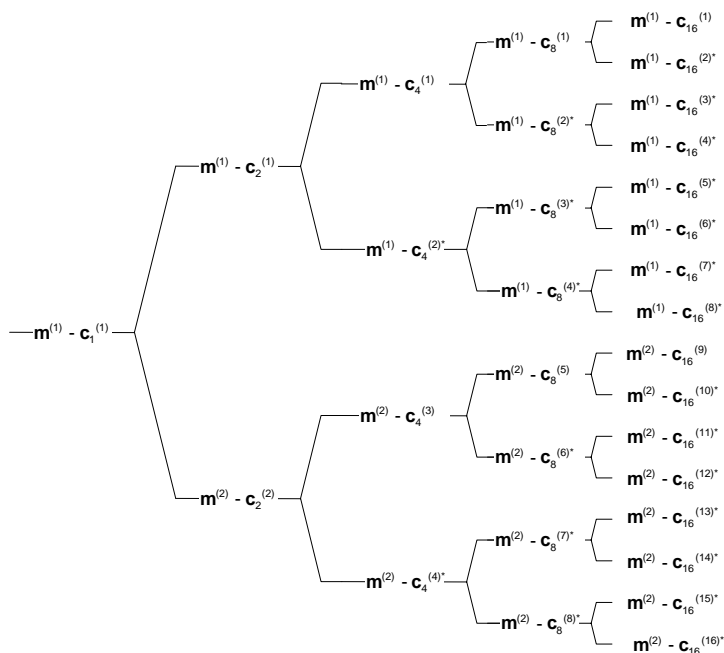
Figure AA.2.8: Association of Midambles to Spreading Codes for K=2
