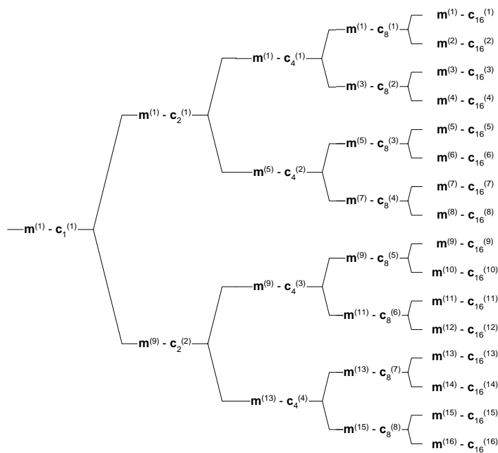
Figure AA.2.1: Association of Midambles to Spreading Codes for K=16
