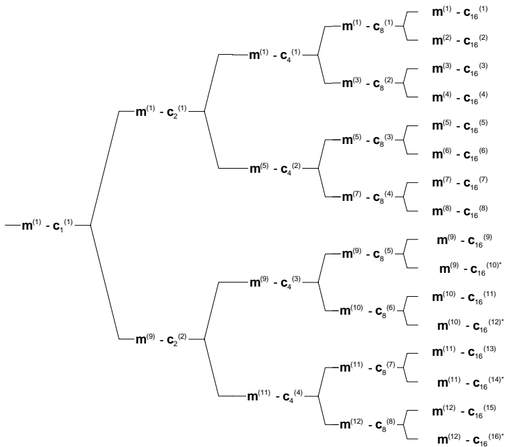
Figure AA.2.3: Association of Midambles to Spreading Codes for K=12
