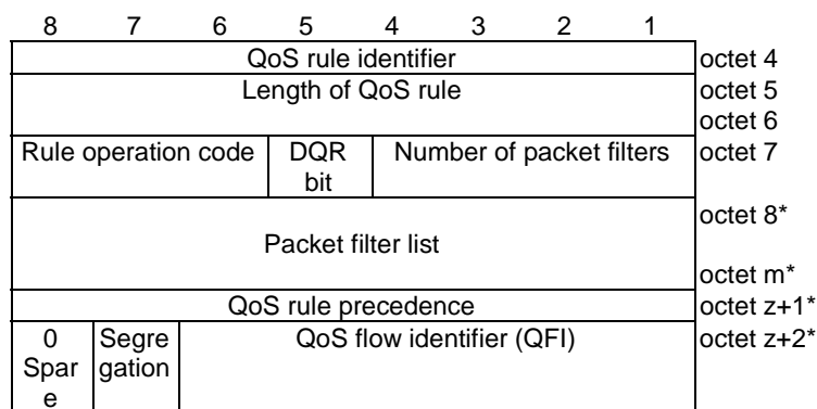
Figure 9.11.4.13.2: QoS rule (u=z+2)
