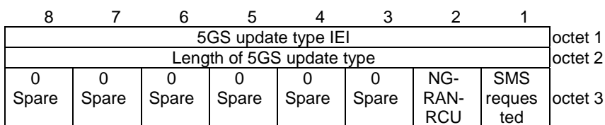
Figure 9.11.3.9A.1: 5GS update type information element
